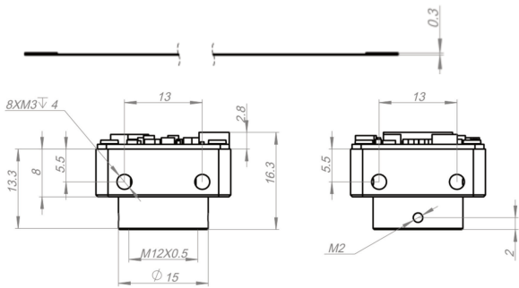
M12传感器板尺寸:
