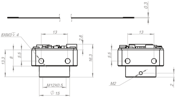
M12传感器板尺寸:
