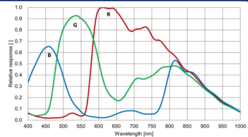
JHEM304GC
